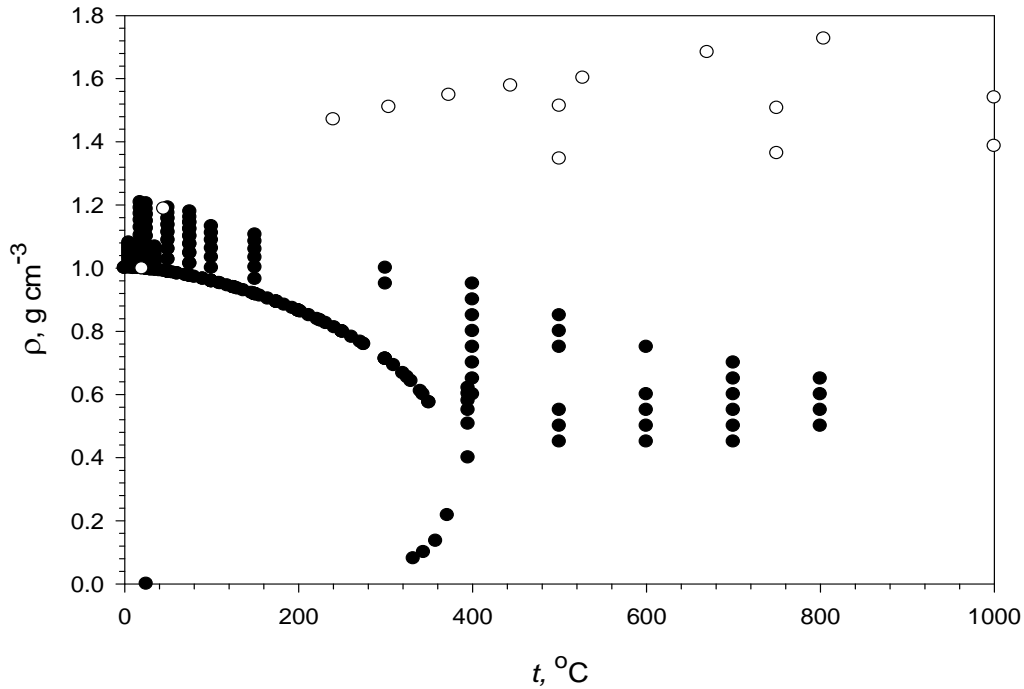
Figure 1. The temperature-density regions of the available experimental K_w data: ● - points used in the fitting procedure, ○ - points that were not used for fitting.
